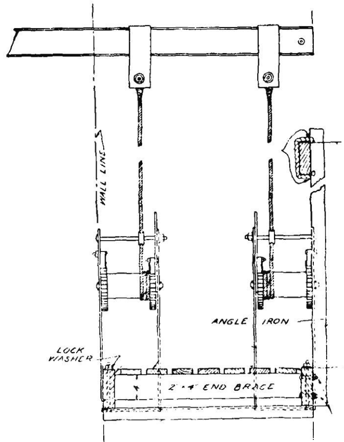
End View of Suspended Scaffold.
