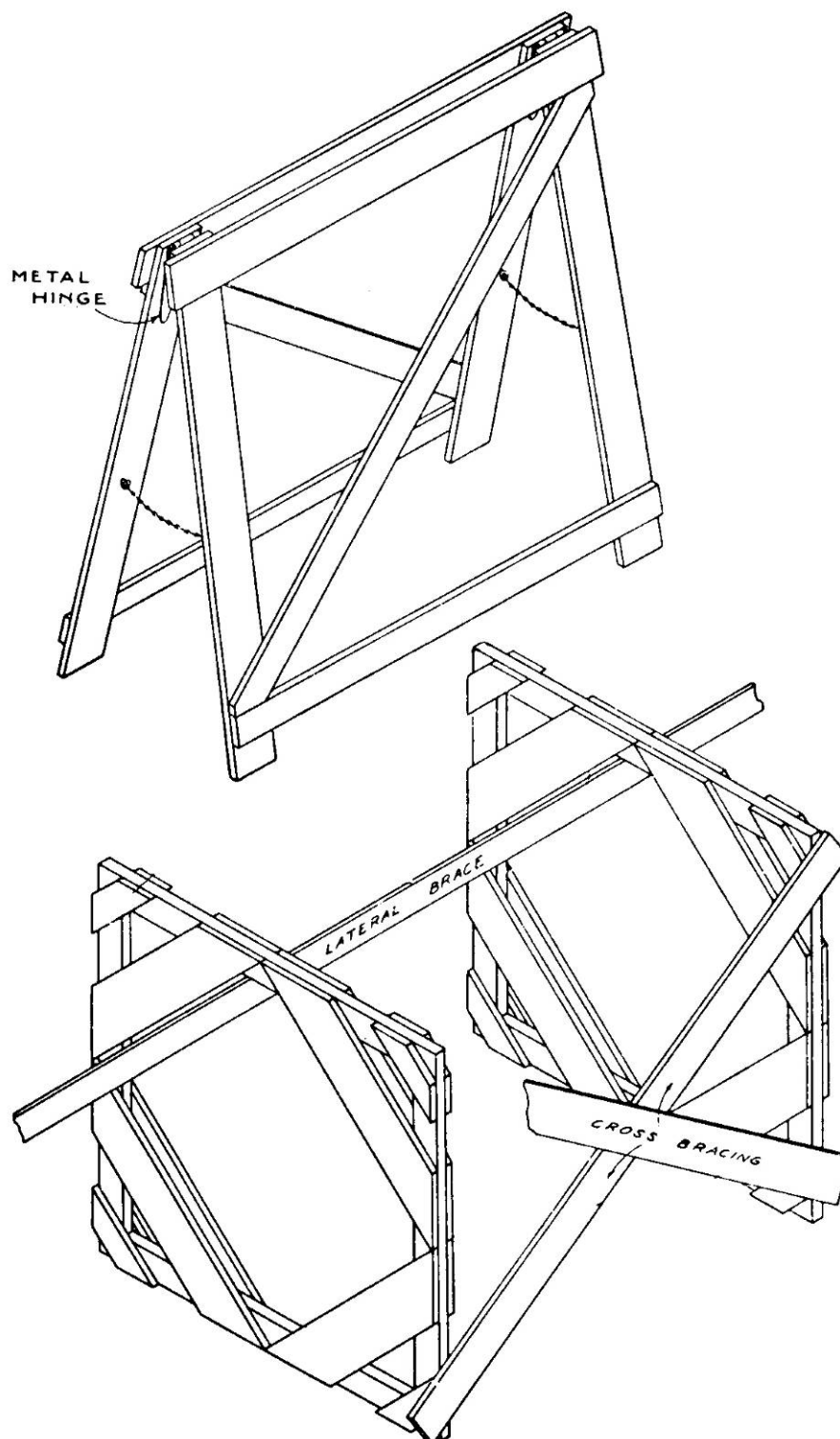
Masons' Square Scaffold Frame.
