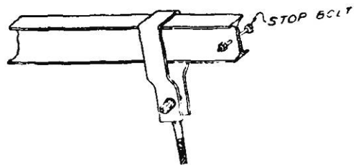
Suspended Scaffold—Thrustout.
