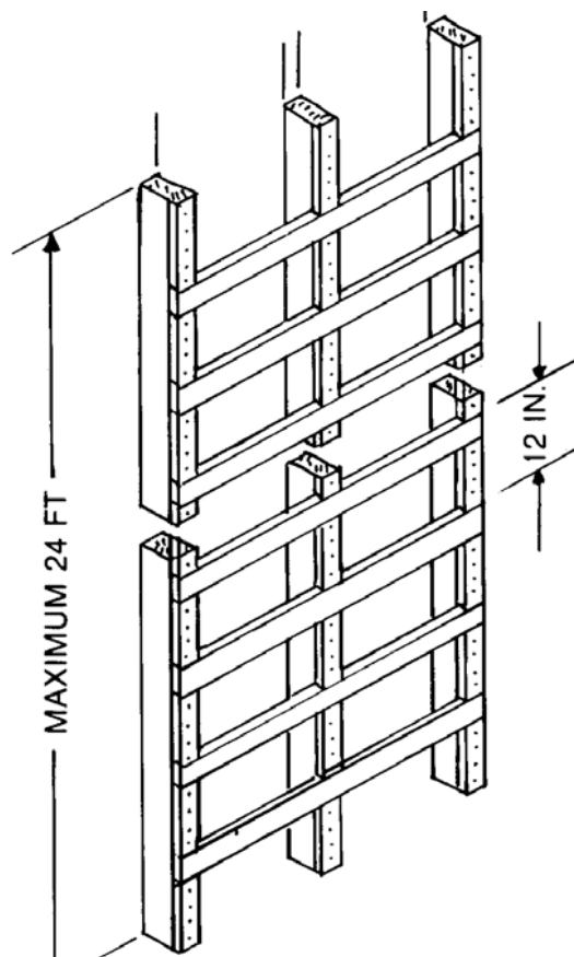
Example 11-2. Double cleat ladder.
