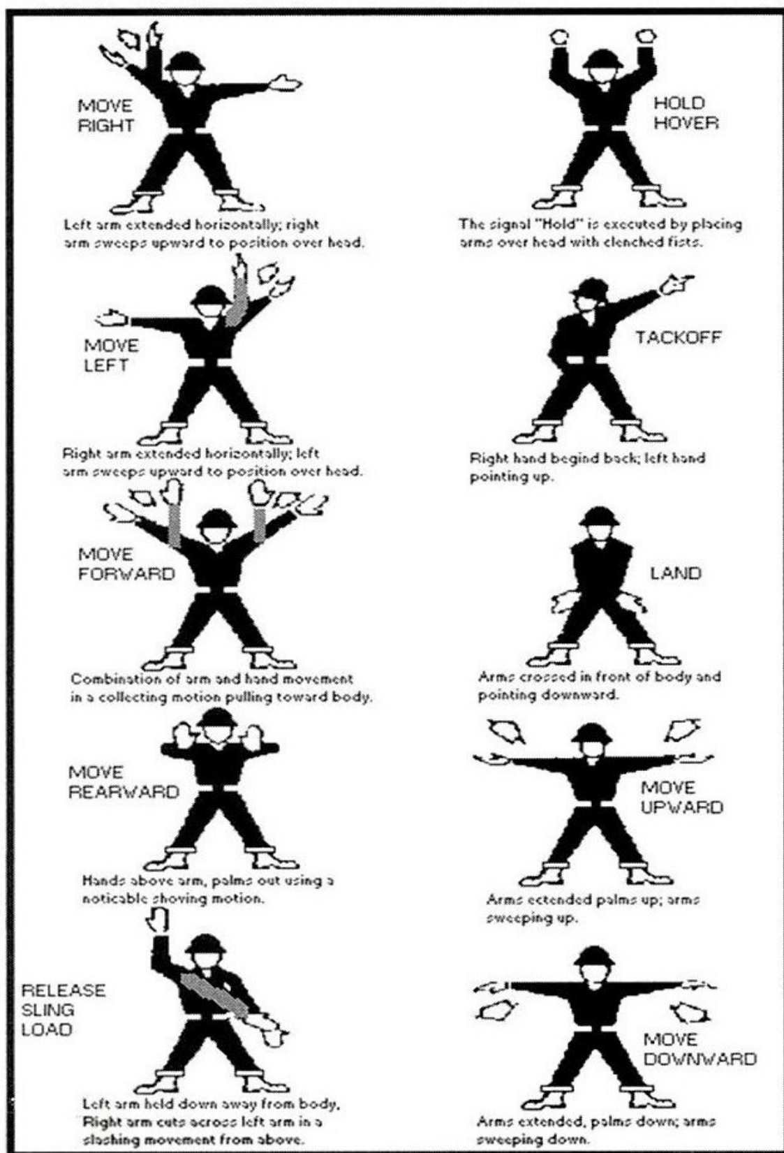
ILLUSTRATION 28-1 HELICOPTER HAND SIGNALS
